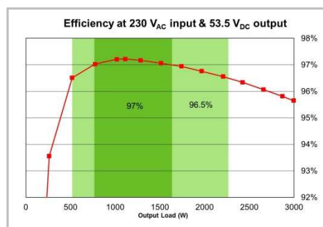
Efficiency vs load plot
