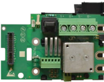
Battery bulk feed with shunt and contactor in positive leg. (241120.912 – 12 VDC only) (241120.914 – 24 - 48 VDC)
