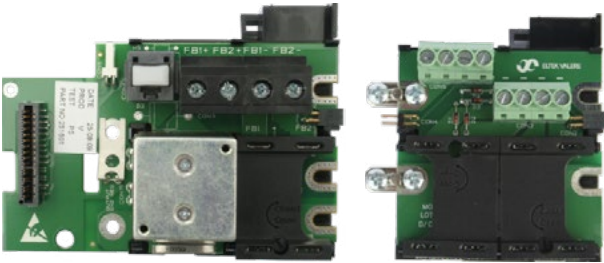
Load distribution with sockets for 4 breakers (241120.920)
